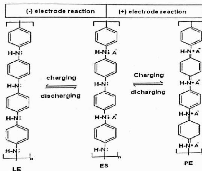
Figure 2: Schematic diagram for the structural changes of PANi backbone during charge-discharge process
